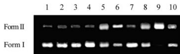
Figure 6. Electrophoresis separation of supercoiled circular \phi X174 RFI DNA (form I) and relaxed circular DNA (form II) after treatment of form I DNA with the osmium complexes 4 and 5 ; lanes 1, 3, 5, 7 were run in the dark, the remaining ones involved UV light irradiation; lane 1, DNA alone (dark, pH = 7.0); lane 2, DNA alone (pH = 7.0); lane 3, DNA alone (pH = 5.0); lane 4, 4 (1000 \mu M, pH = 7.0, dark); lane 5, 4 (1000 \mu M, pH = 7.0); lane 6, 4 (1000 \mu M, pH = 5.0); lane 7, 5 (1000 \mu M, pH = 7.0, dark); lane 8, 5 (1000 \mu M, pH = 7.0); lane 9, 5 (1000 \mu M, pH = 5.0); lane 10, 5 (1.0 \mu M, pH = 5.0)
